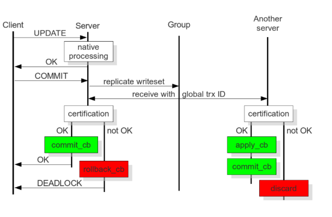
Figure 3.1: Image source: Galera documentation - HOW CERTIFICATION-BASED REPLICATION WORKS
