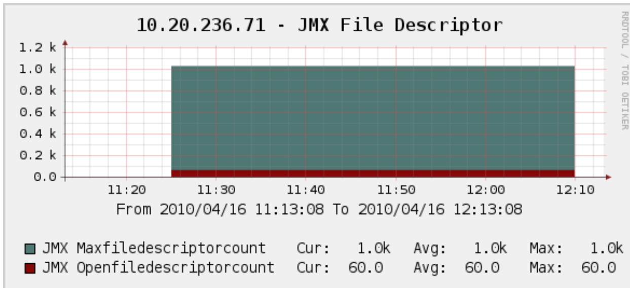
The file descriptors used by the JMX process.
